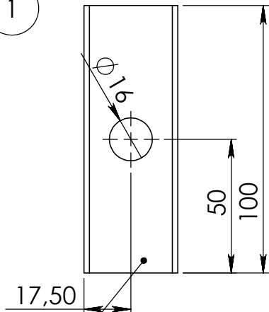
Tube carré 35x35x2
