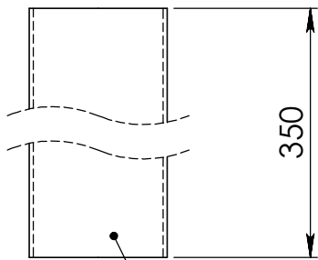
Tube \phi 100x3mm
